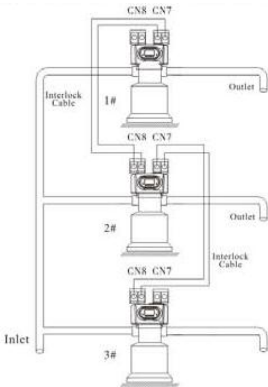
Figure 3-12 Interlock system
